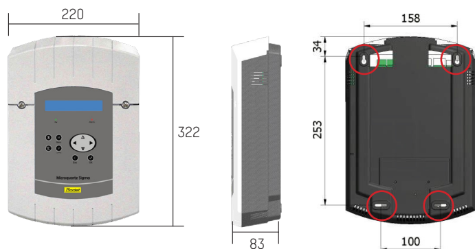
Wall-mounted version
