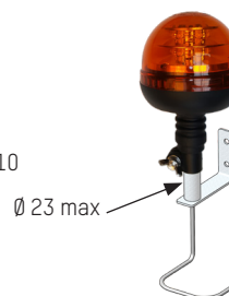
Wall mounting of LED beacon strobe light on wall bracket
