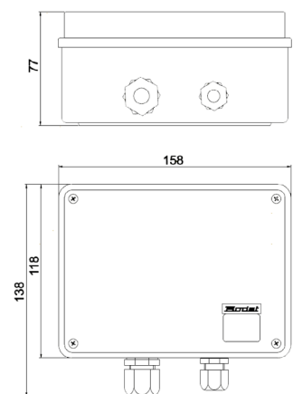
Abmessungen in mm
